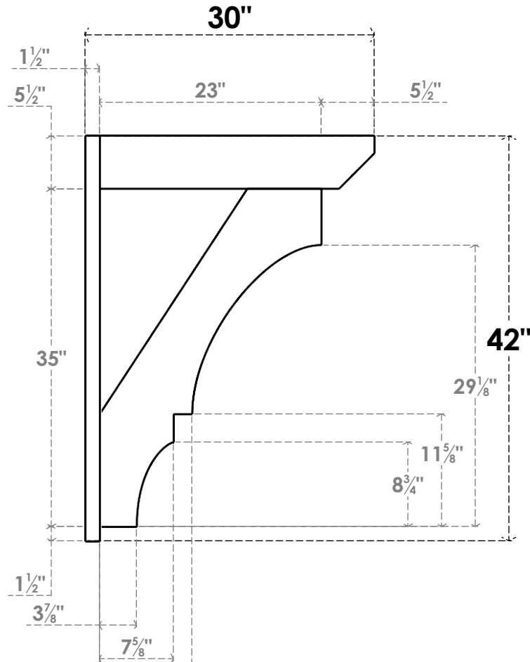
SIDE PROFILE
